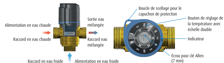
FIGURE 2: VANNE ATM
